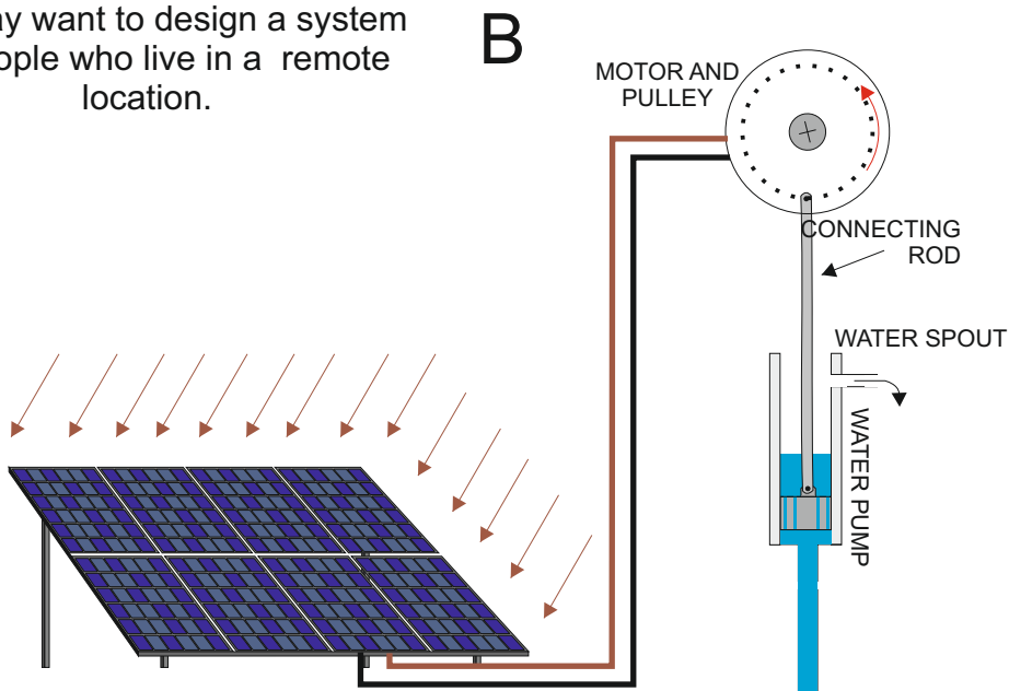
SOLAR POWERED WATER PUMP
