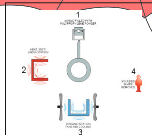
ROTATIONAL MOULDING
