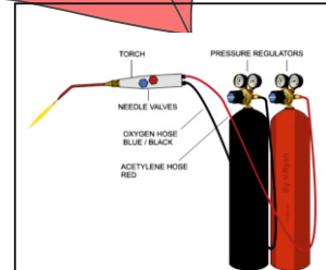
OXYACETYLENE WELDING
