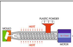
INJECTION MOULDING
