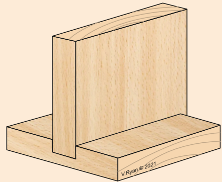
ASSEMBLED VIEW
