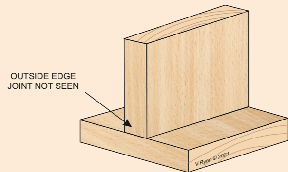
ASSEMBLED VIEW
