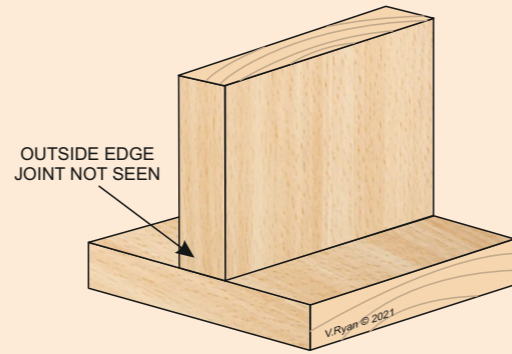
ASSEMBLED VIEW
