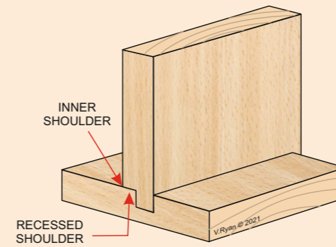
ASSEMBLED VIEW
