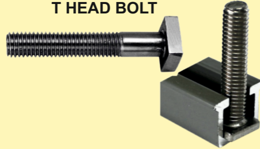
TITANIUM BOLT
