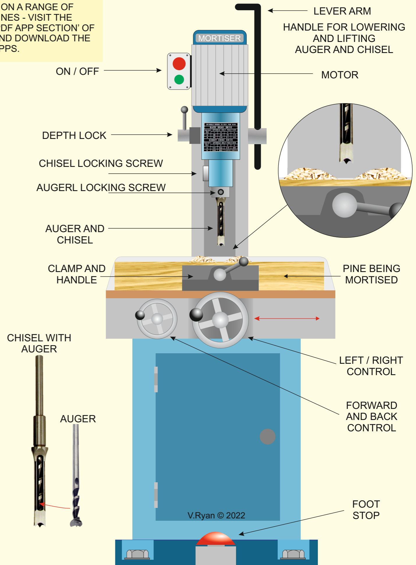
FRONT VIEW
