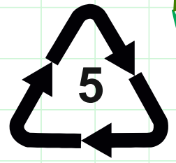
PP Polypropylene
