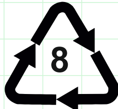
Pb Lead
